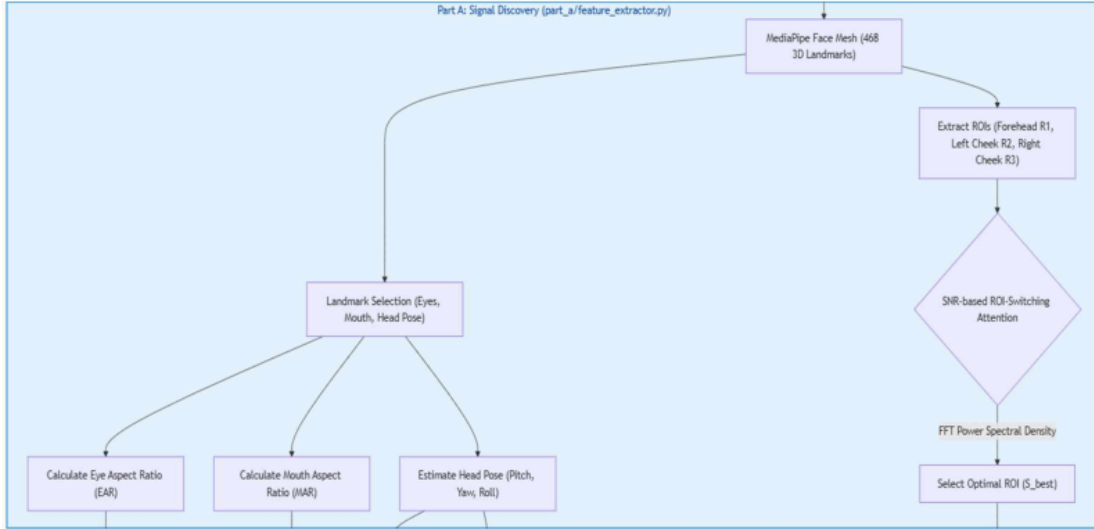
Figure 3.2 SNR-based ROI-Switching Attention Logic.
