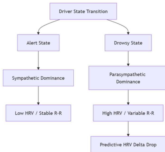
Figure 2.4 Sympathoyagal Balance during Fatigue Transition
